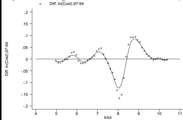
Graph 9b: Cumulated effect of between and within diffusion of the distribution of ln(cost)
