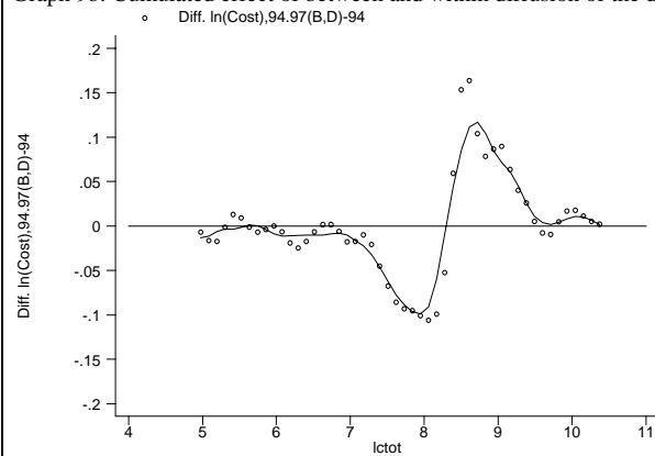
Graph 9c: Effect of changes in unobservable heterogeneity and observable patients' characteristics on the distribution of ln(cost)
